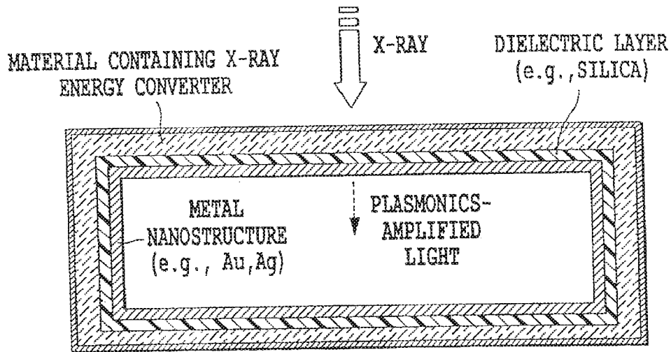
Fig. 28 STERILIZATION SYSTEM 2 WITH PLASMONICS
