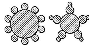
MULTI-NANOPARTICLE STRUCTURES
