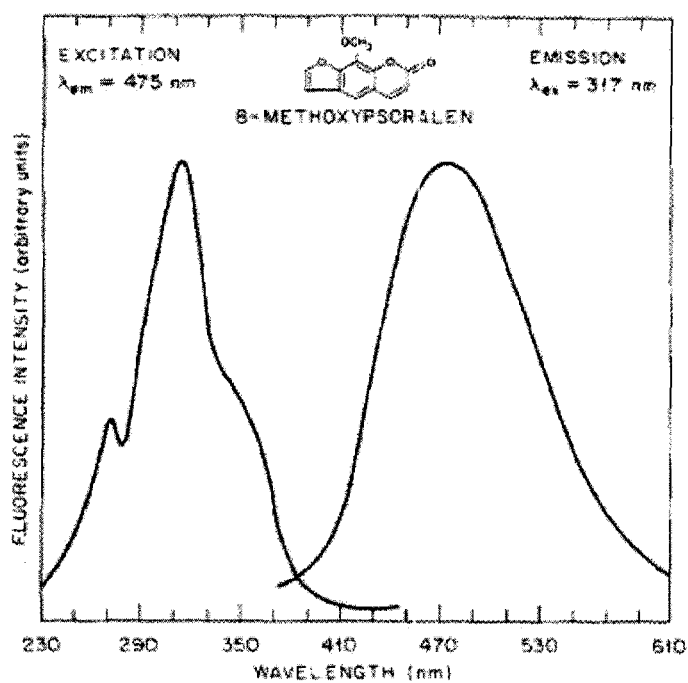
Figure 19. Excitation and Emission Fluorescence Spectra of Psoralens [Source: T. Vo-Dinh et al, J. Agric. Food Chem. , 36, 335 (1988)]
