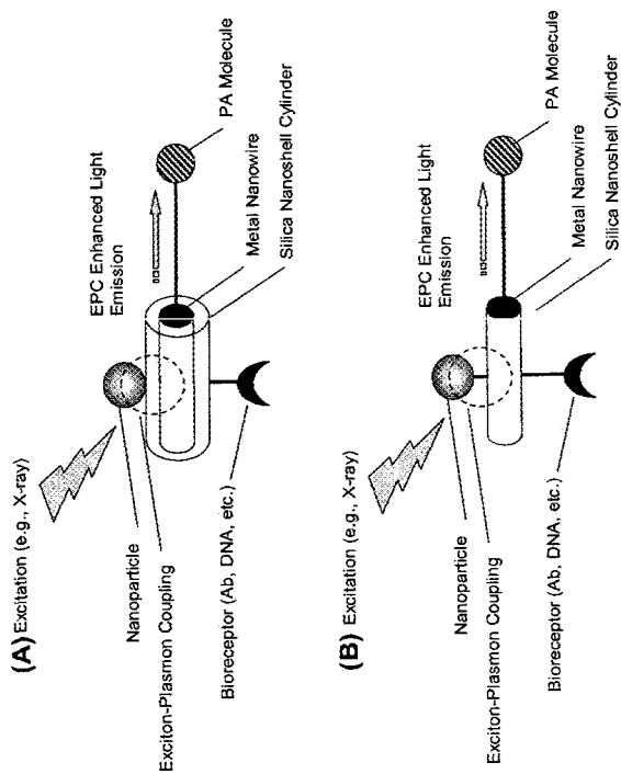
Exciton-Plasmon Coupling (EPC) Between Metal Nanorod and Nanoparticle
