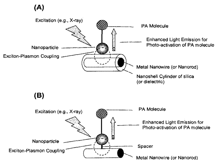
Exciton-Plasmon coupling Between Metal Nanorod and Nanoparticle
