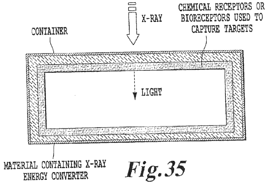
STERILIZATION SYSTEM 9 WITH CHEMICAL RECEPTORS OR BIORECEPTORS
