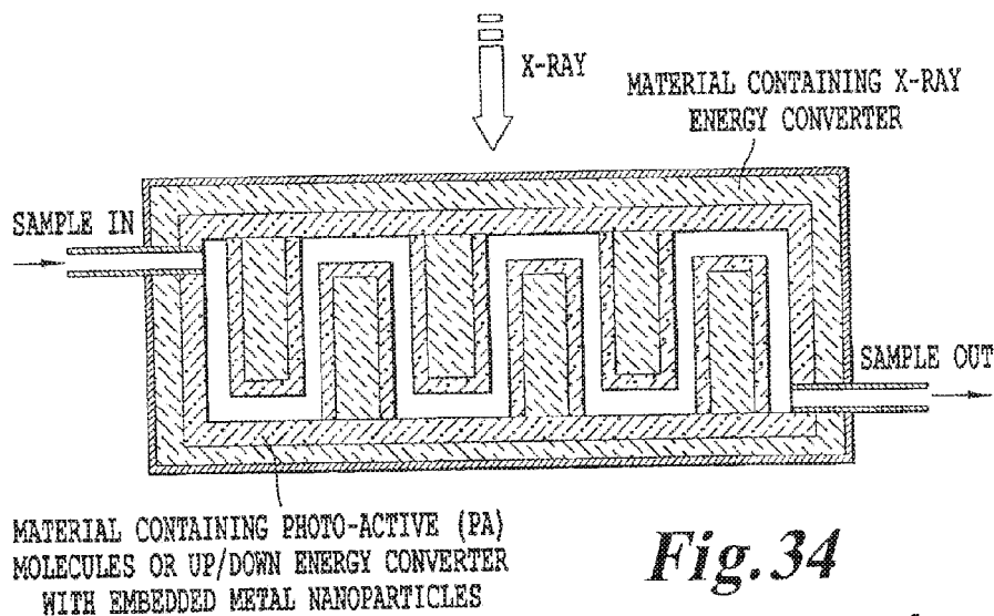
STERILIZATION SYSTEM 8 WITH PLASMONICS
