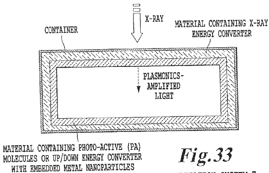
STERILIZATION SYSTEM 7 WITH PLASMONICS
