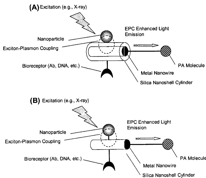
Figure 32. Embodiments of EPEP Probes Having NPs, NWs, NRs and Bioreceptors
