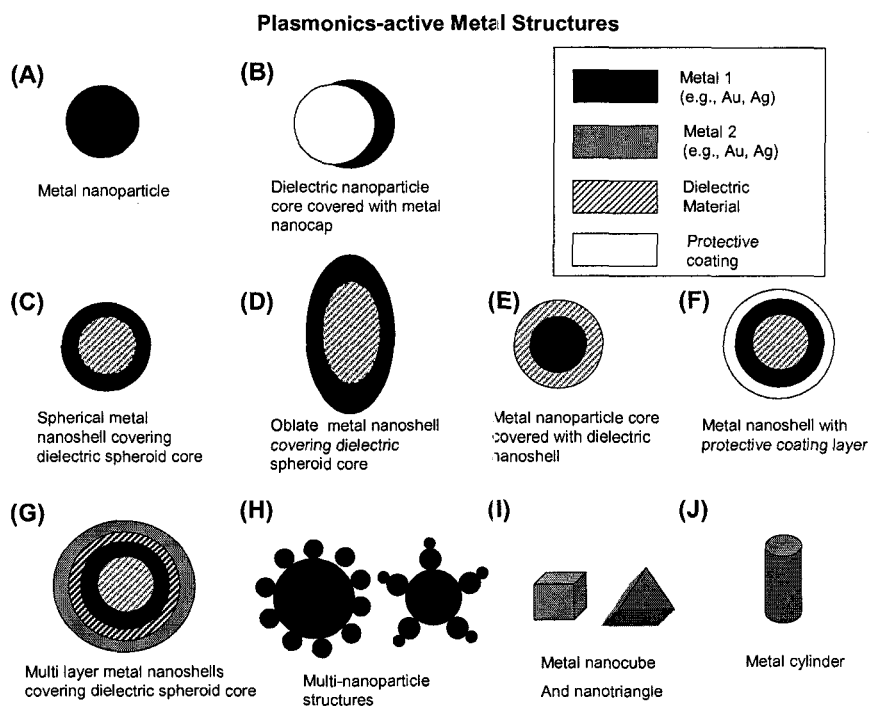
Figure 9. Plasmonics-active Nanostructures
