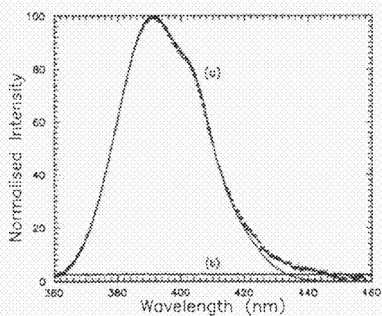
Figure 2. Curves a, the XEOL spectrum of BaFBr:Eu. The dashed curve is the observed spectrum and the continuous curve passing through the observed spectrum is the fitted spectrum. Curve b, the XEOL spectrum of pristine BaFBr.
