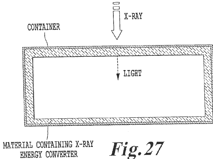
STERILIZATION SYSTEM 1
