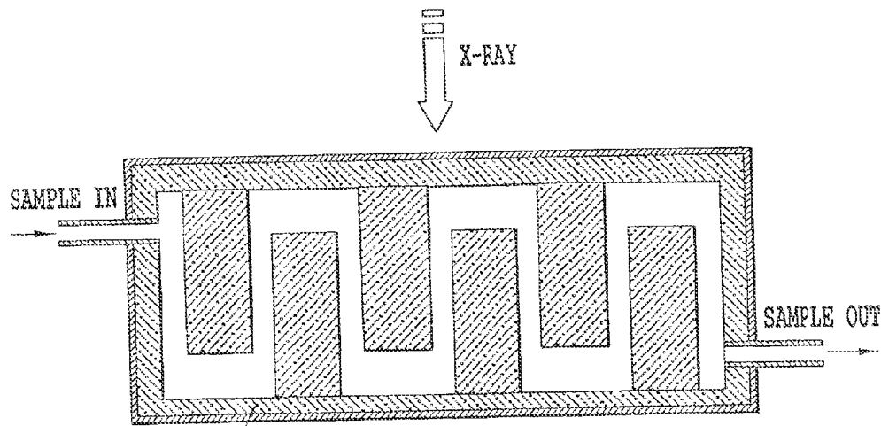
Fig. 32 STERILIZATION SYSTEM 6 WITH PLASMONICS
