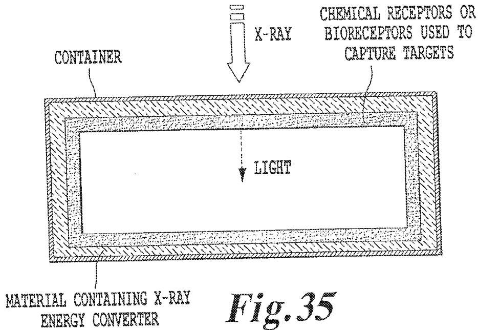
STERILIZATION SYSTEM 9 WITH CHEMICAL RECEPTORS OR BIORECEPTORS
