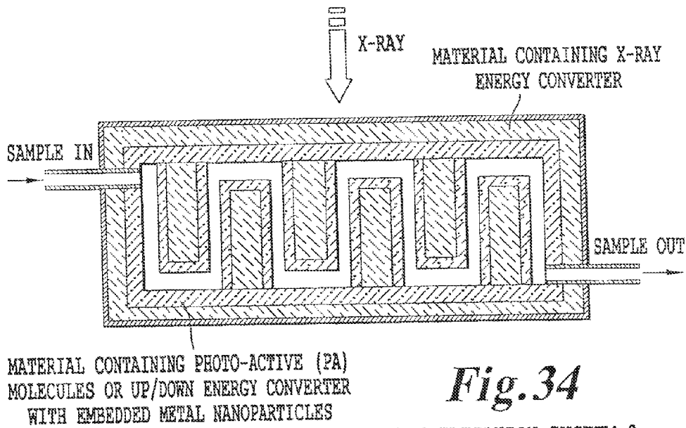
STERILIZATION SYSTEM 8 WITH PLASMONICS
