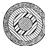
X-RAY CONVERTER NANOPARTICLE COVERED WITH DIELECTRIC LAYER AND METAL NANOSHELL WITH PROTECTIVE COATING LAYER
