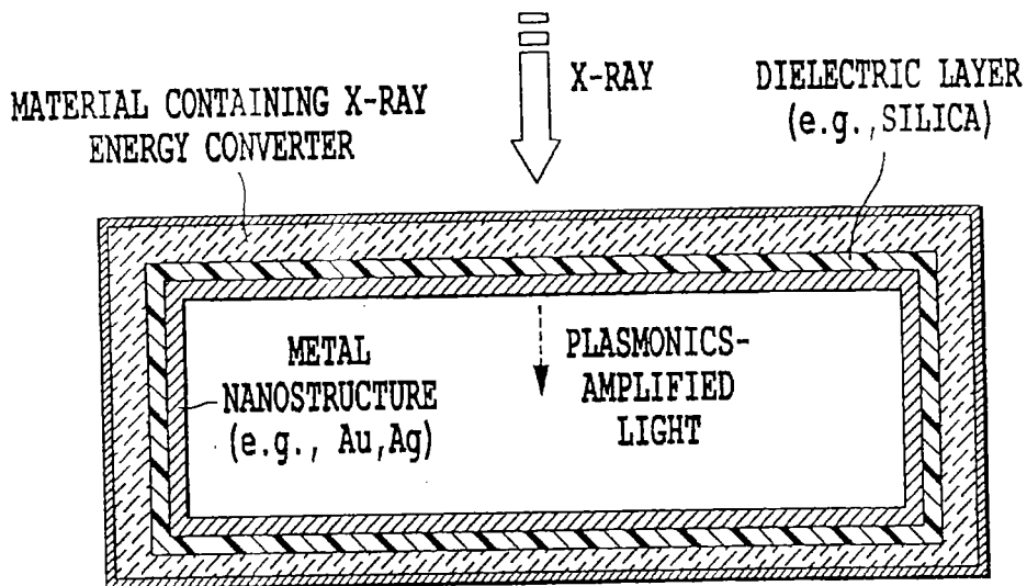
Fig. 28 STERILIZATION SYSTEM 2 WITH PLASMONICS
