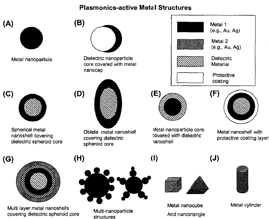
Figure 9. Plasmonics-active Nanostructures
